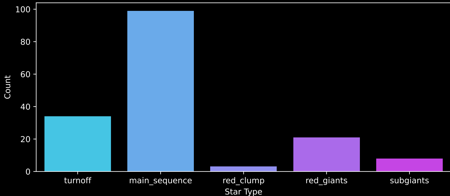
APOGEE DR17 Field: [042+87_MGA] Count plot of Star Type
