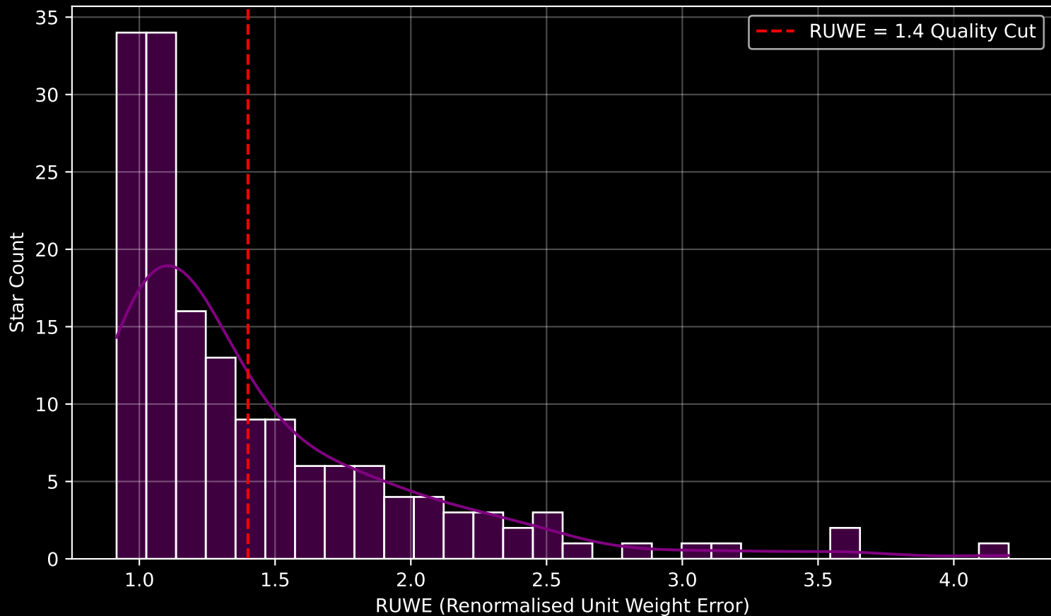
GAPOGEE DR17 Field [042+87_MGA] RUWE Distribution (n= 159)
