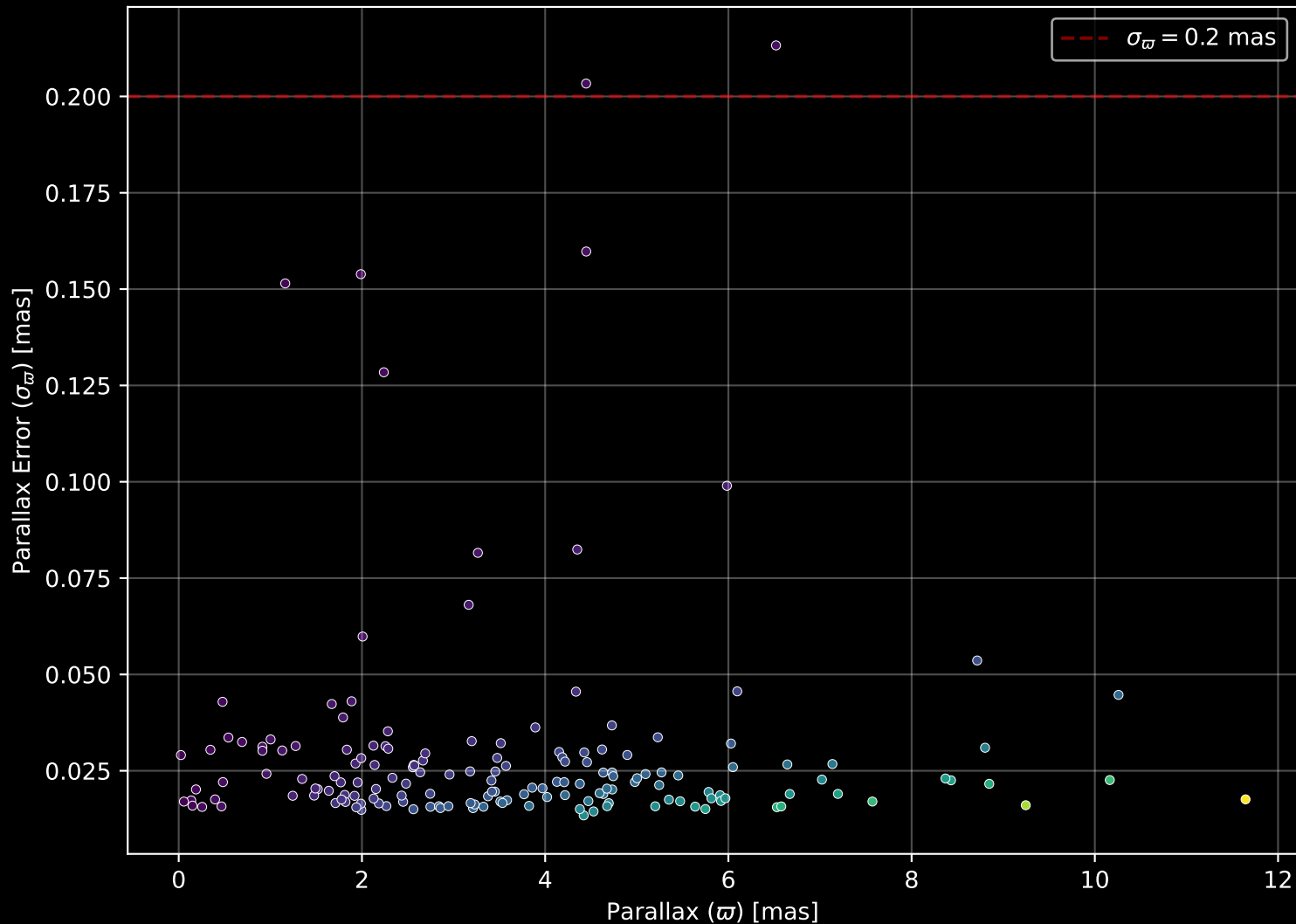
APOGEE DR17 Field: [042+87_MGA] Parallax Quality (n= 165)
