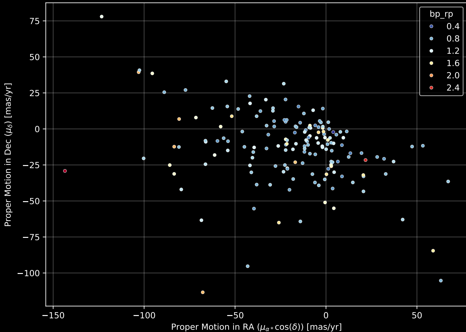
APOGEE DR17 Field: [042+87_MGA] Proper Motion Diagram (n= 165)
